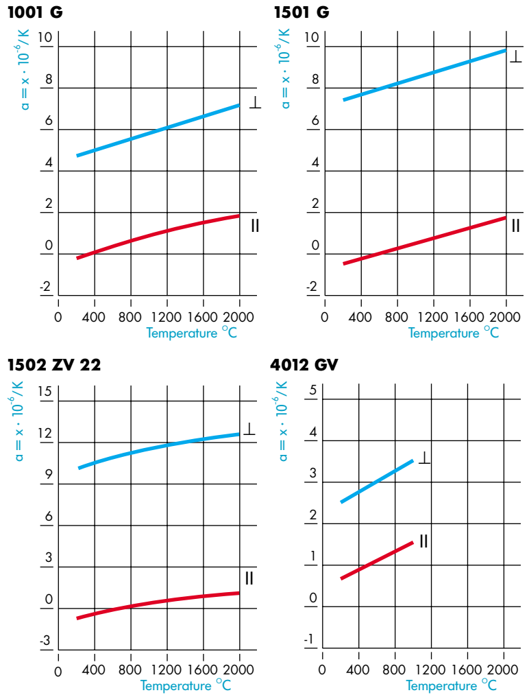
Figure 4 Linear coefficient of thermal expansion ( \alpha ) of various ®SIGRABOND sheet materials
