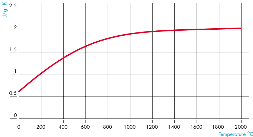
Figure 9 Specific heat of *SIGRABOND 1001 G
