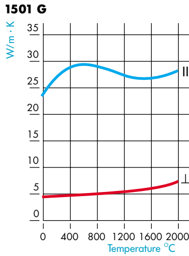
Figure 6 Thermal conductivity of various ® SIGRABOND grades
