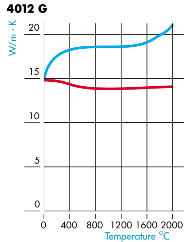
Figure 7 Axial thermal conductivity of ® SIGRABOND pipes
